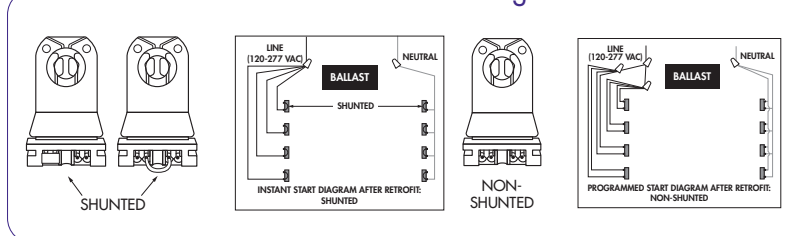
Double Ended Wiring
