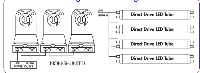
Single Ended Wiring
