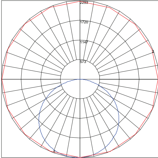
Maximum Candela = 2293.1 Located At Horizontal Angle = 270, Vertical Angle = 3.5 # 1 - Vertical Plane Through Horizontal Angles (270 - 90) (Through Max. Cd.) # 2 - Horizontal Cone Through Vertical Angle (3.5) (Through Max. Cd.)
