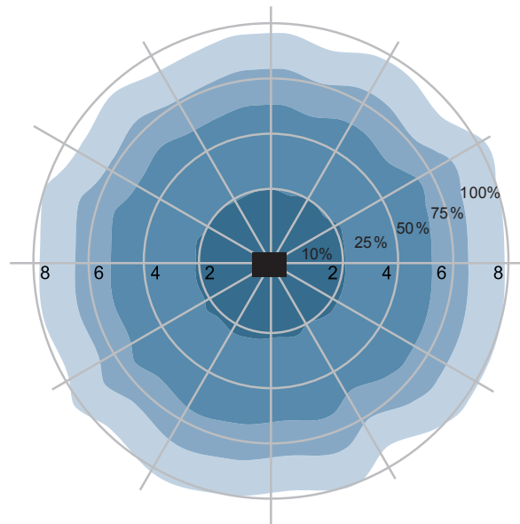
Ceiling Mounting Pattern (Unit: m)
