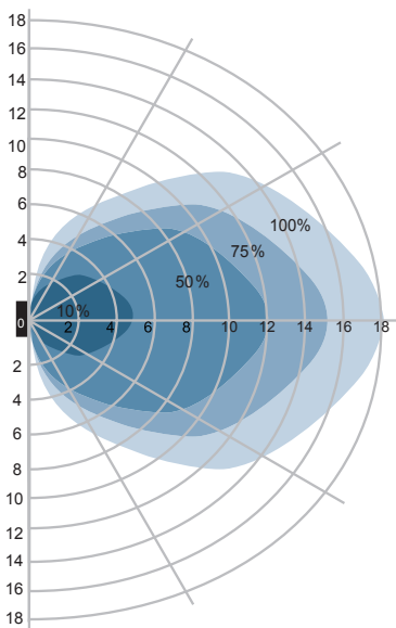
Wall Mounting Pattern (Unit: m)
