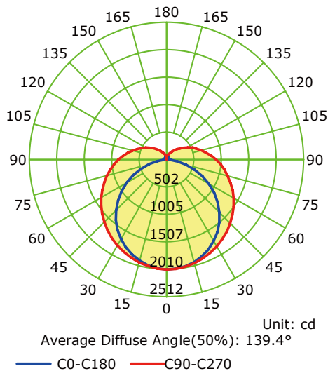
LLB56001 Luminous Intensity Distribution Curve
